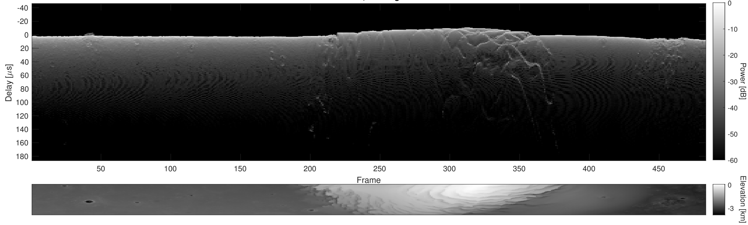
Orbit 5481, Cluttergram
