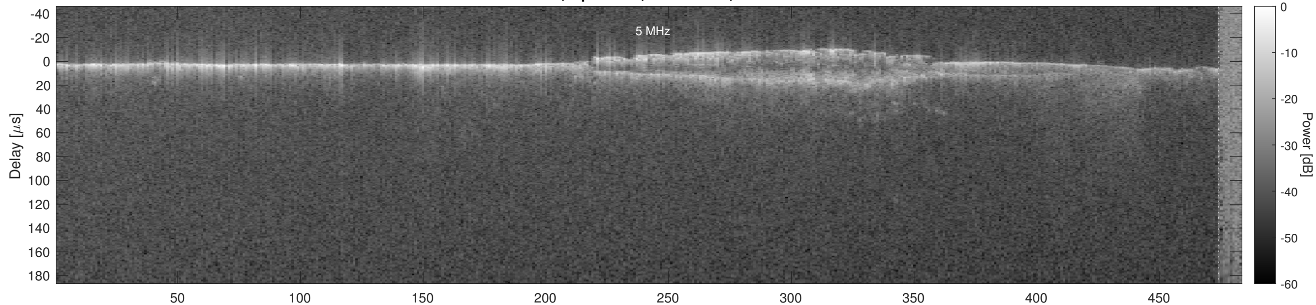
Orbit 5481, Optimized, No Window, Channel 2
