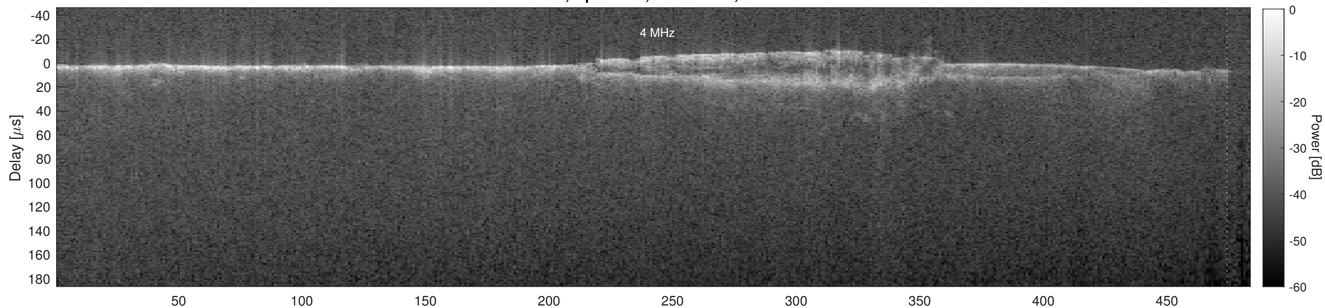
Orbit 5481, Cluttergram
