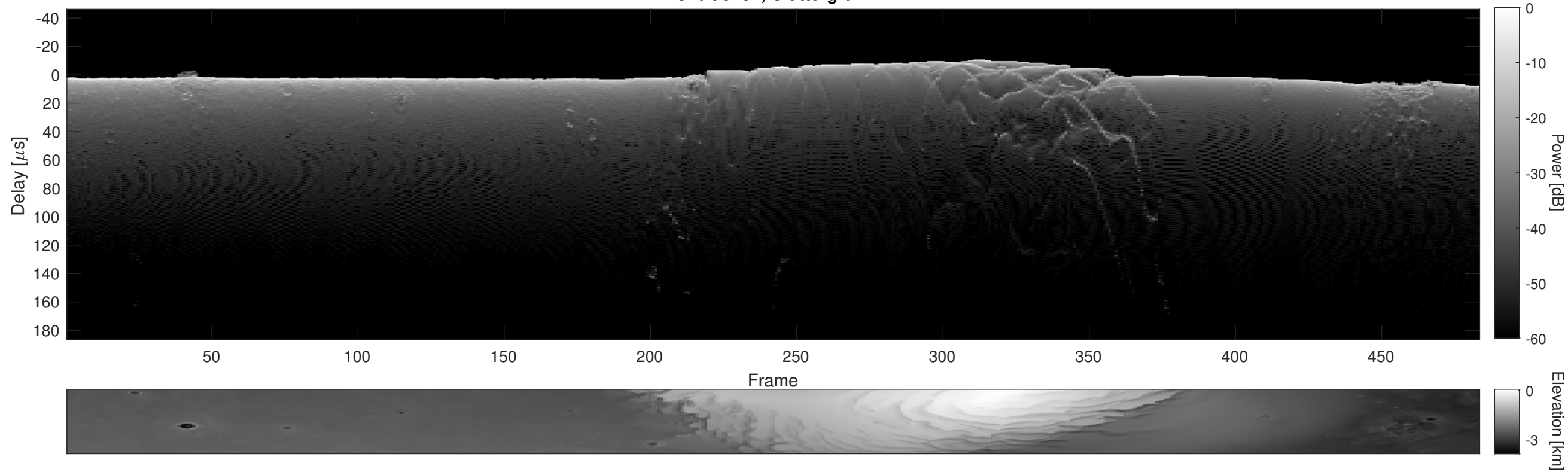
Orbit 5481, Cluttergram
