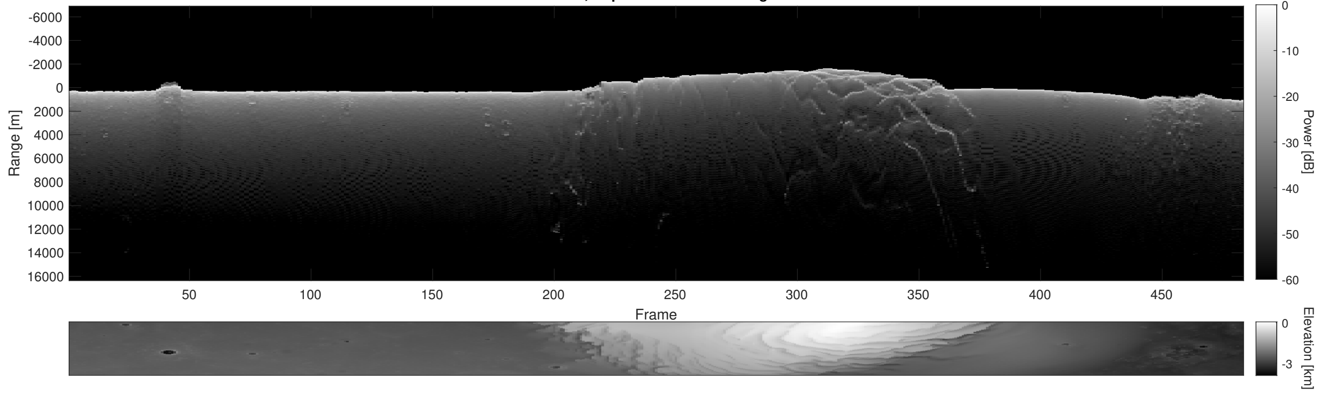
Orbit 5481, Depth-Corrected Cluttergram
