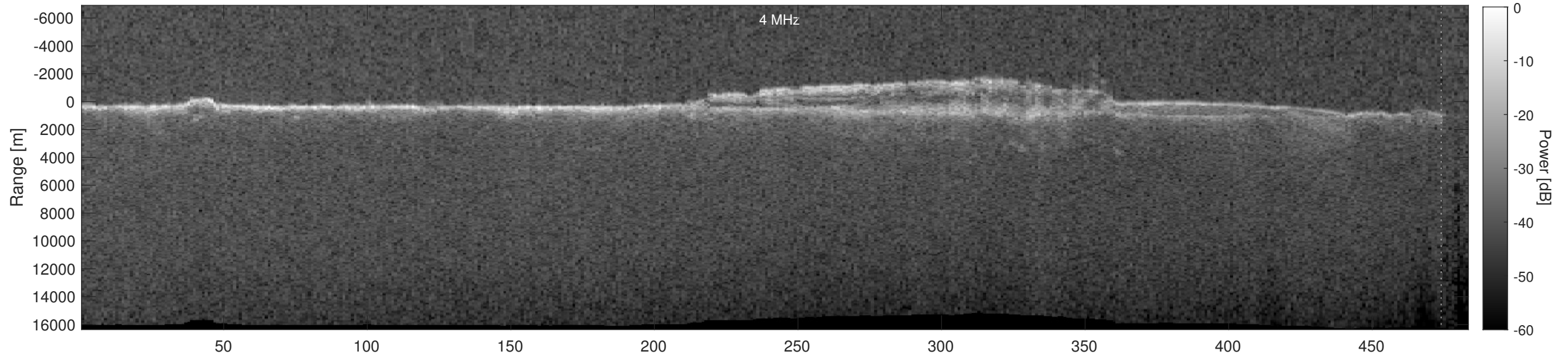
Orbit 5481, Depth-Corrected Cluttergram
