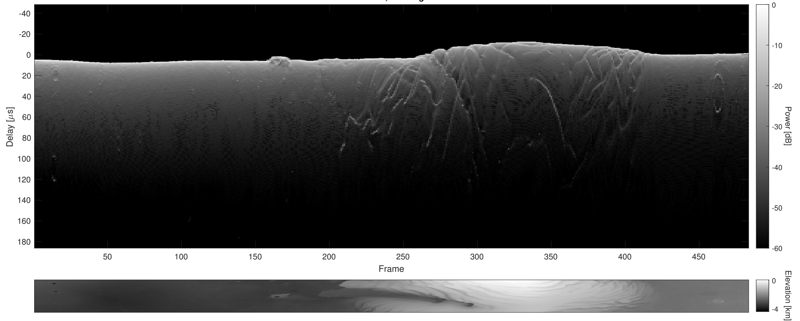
Orbit 5482, Cluttergram
