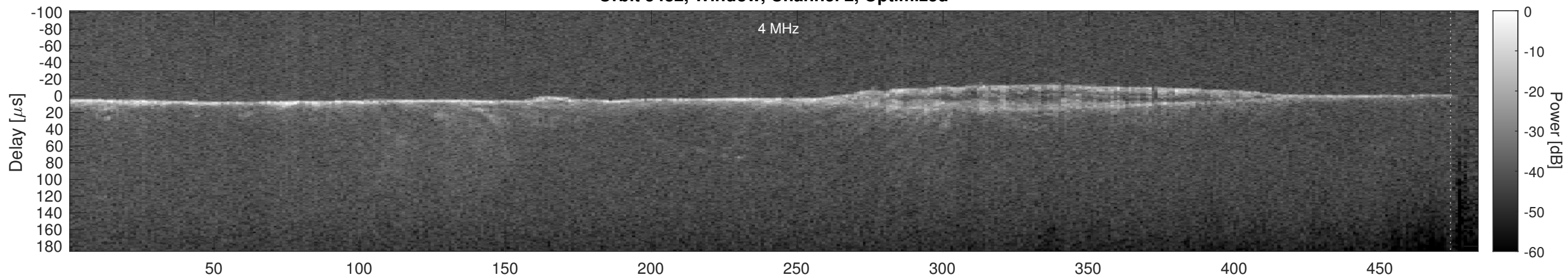
Orbit 5482, Cluttergram
