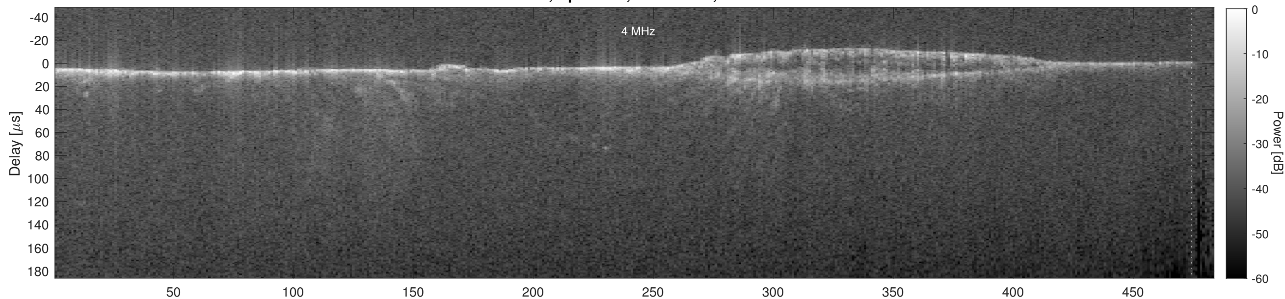
Orbit 5482, Cluttergram
