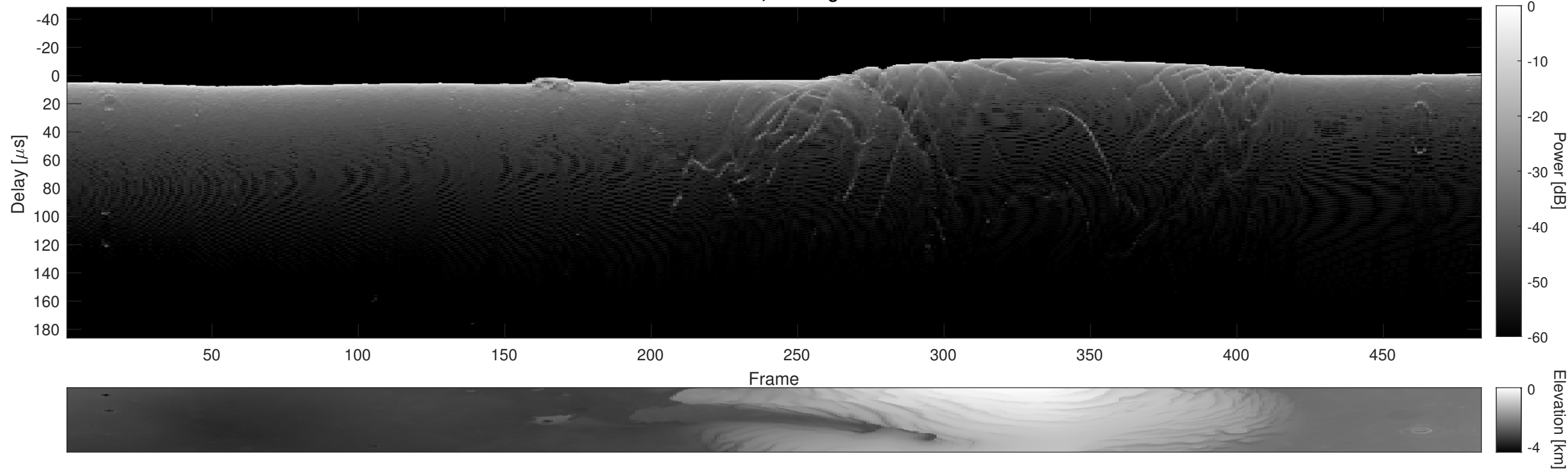
Orbit 5482, Cluttergram
