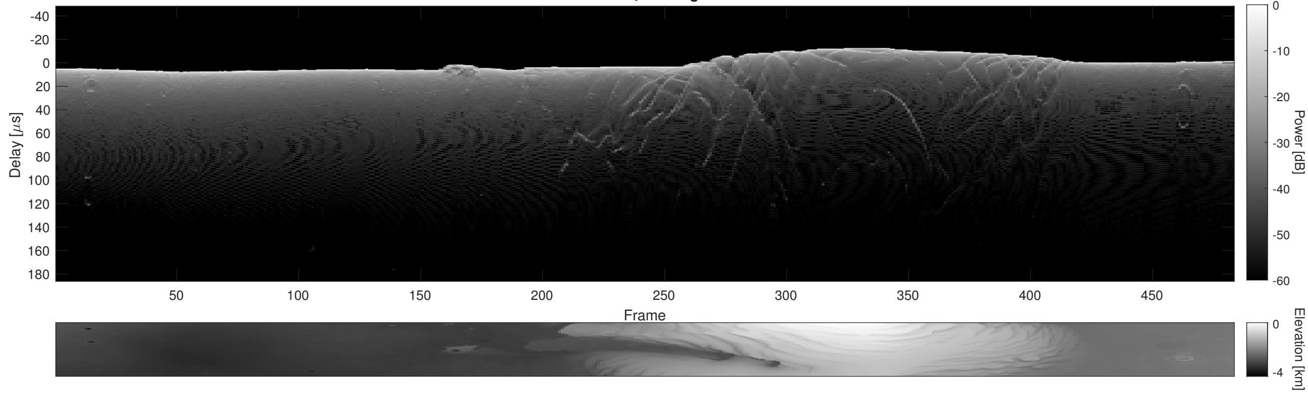
Orbit 5482, Cluttergram
