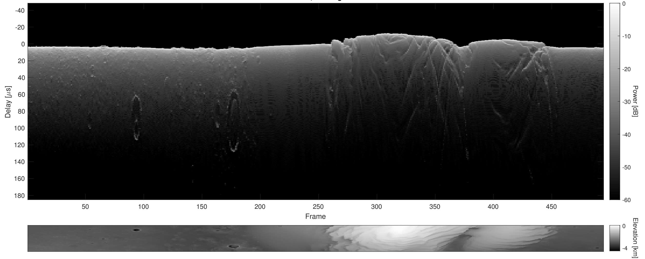
Orbit 5483, Cluttergram
