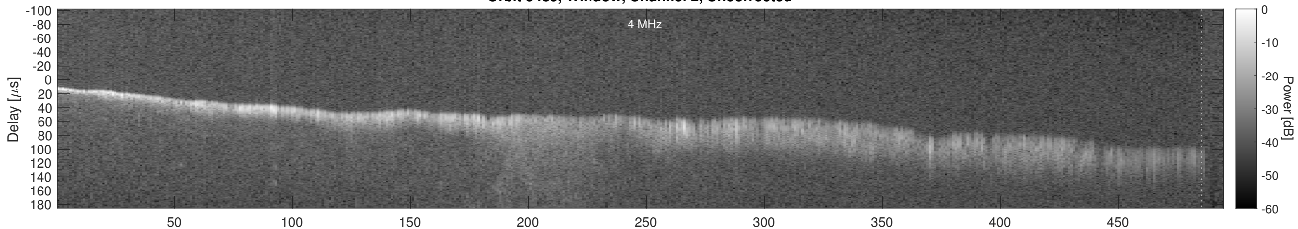
Orbit 5483, Window, Channel 2, Chapman
