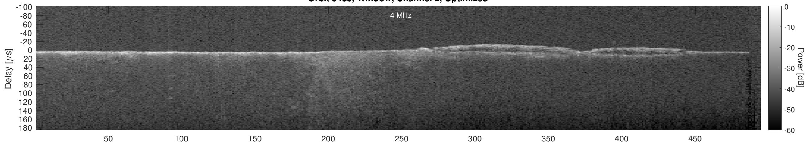
Orbit 5483, Cluttergram
