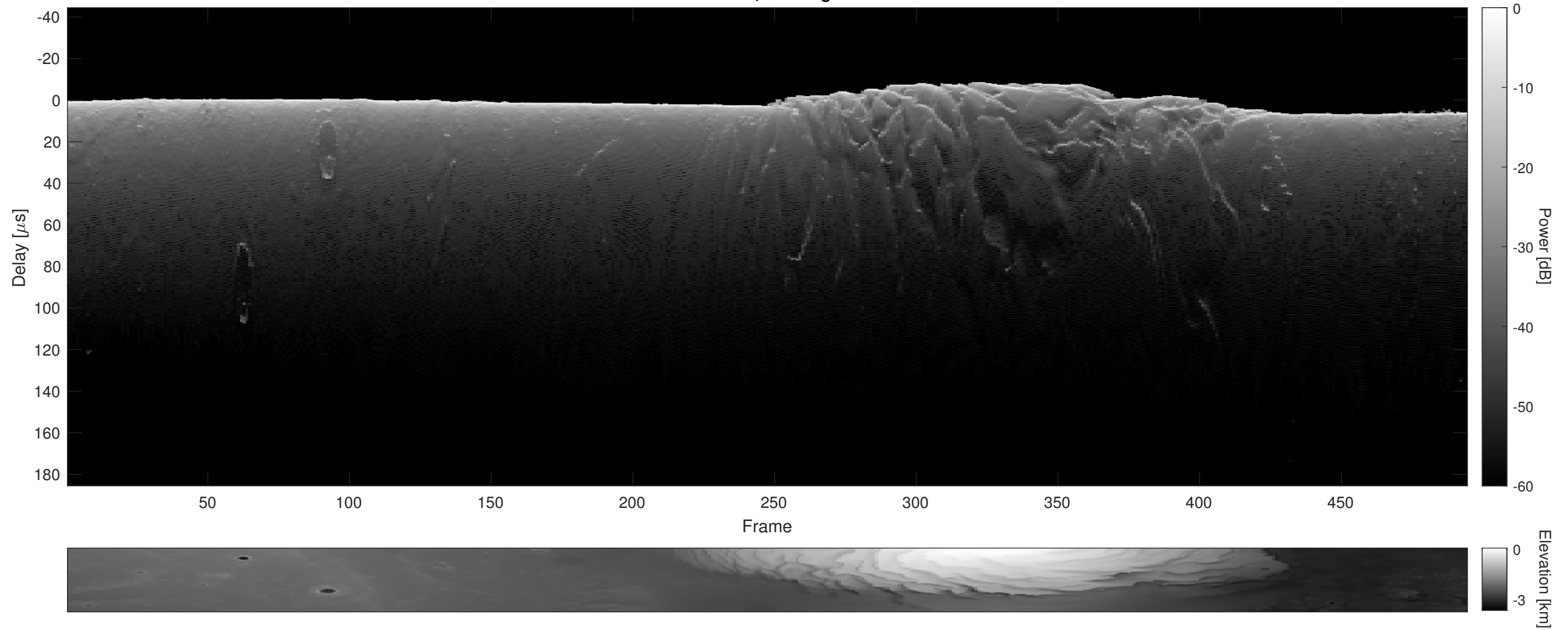
Orbit 5484, Cluttergram
