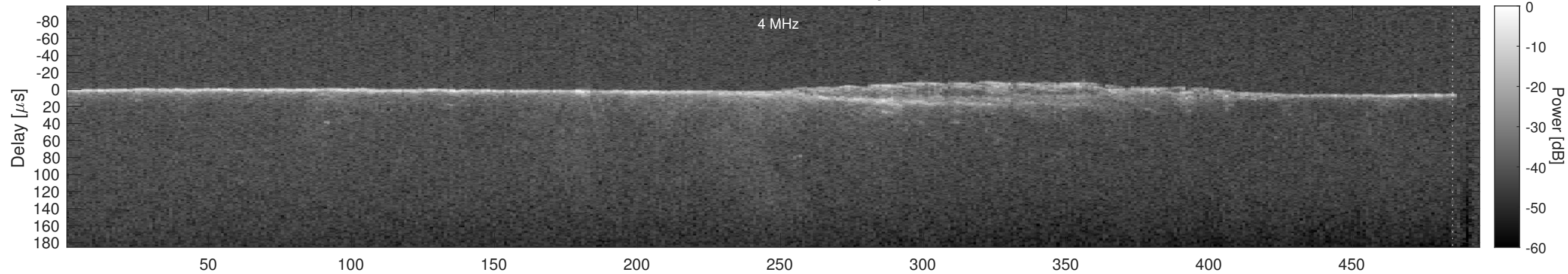
Orbit 5484, Cluttergram
