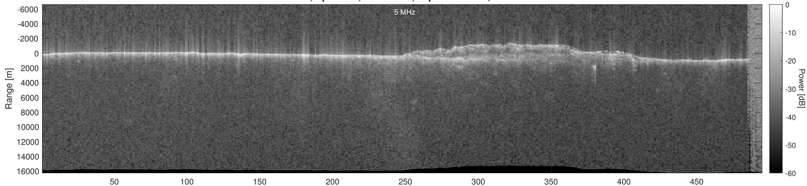
Orbit 5484, Optimized, No Window, Depth-Corrected, Channel 2
