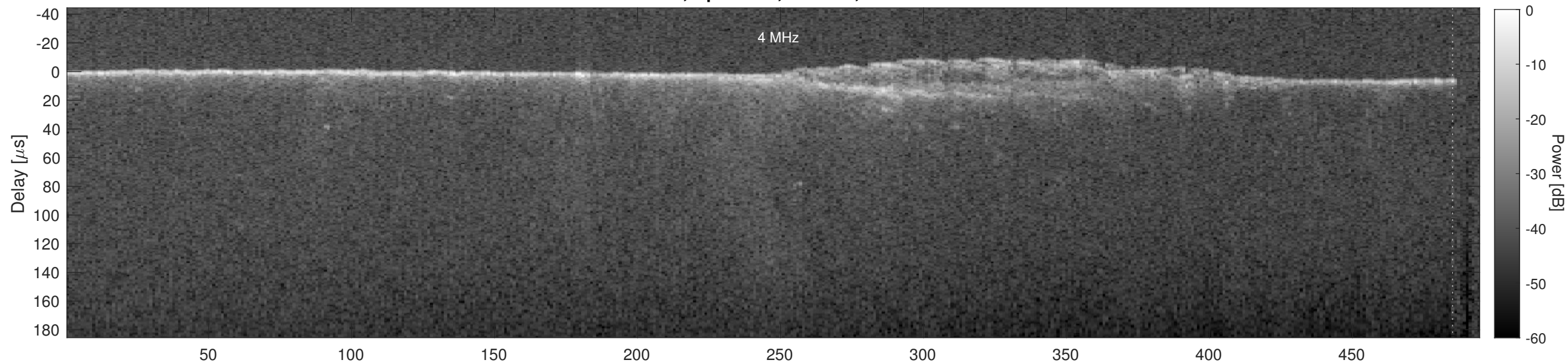
Orbit 5484, Cluttergram
