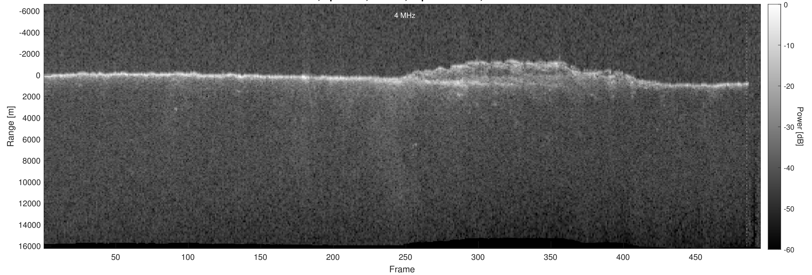
Orbit 5484, Optimized, Window, Depth-Corrected, Channel 2
