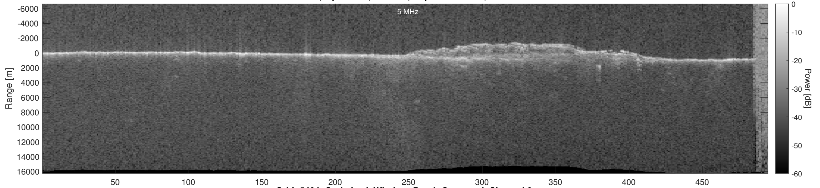
Orbit 5484, Optimized, Window, Depth-Corrected, Channel 2
