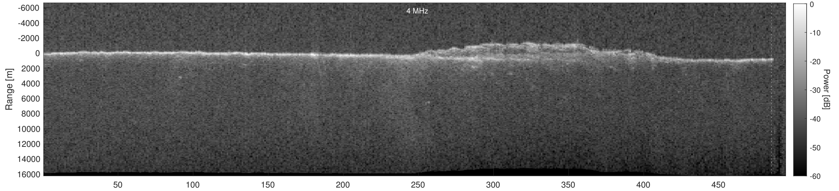
Orbit 5484, Depth-Corrected Cluttergram
