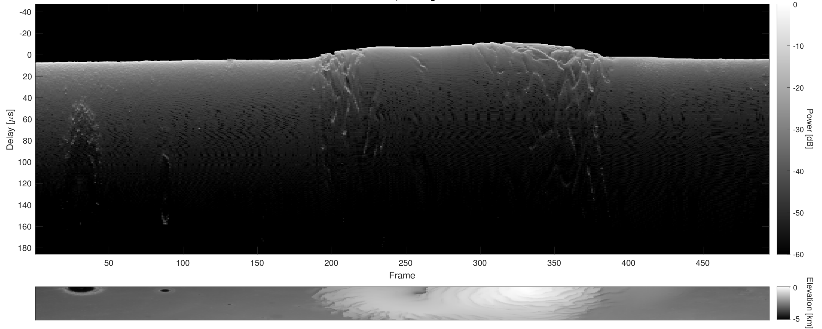
Orbit 5485, Cluttergram
