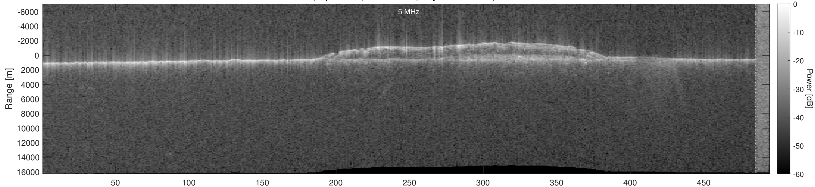
Orbit 5485, Optimized, No Window, Depth-Corrected, Channel 2
