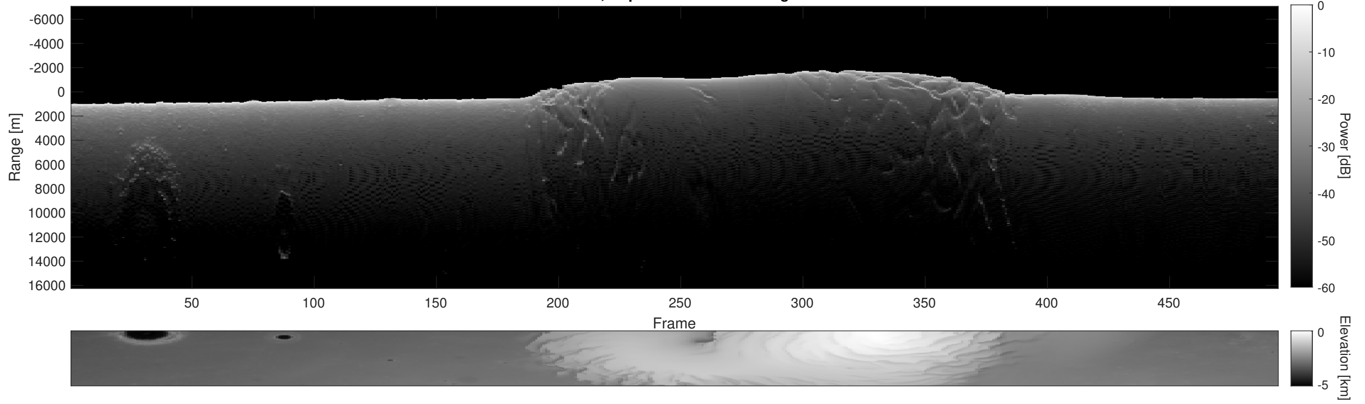
Orbit 5485, Depth-Corrected Cluttergram
