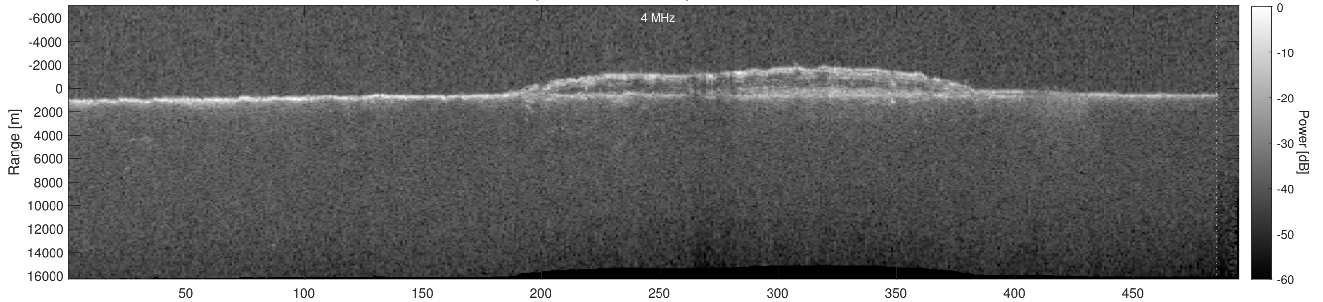
Orbit 5485, Depth-Corrected Cluttergram
