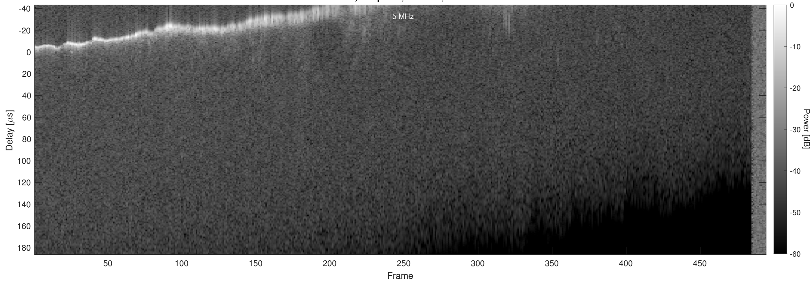
Orbit 5486, Chapman, Window, Channel 2
