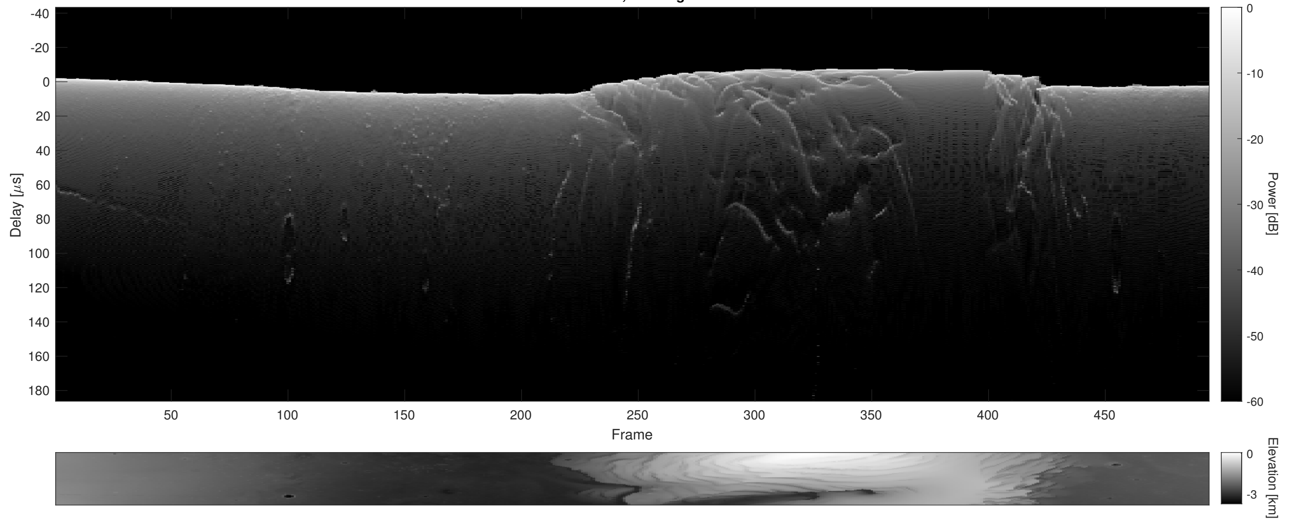
Orbit 5486, Cluttergram
