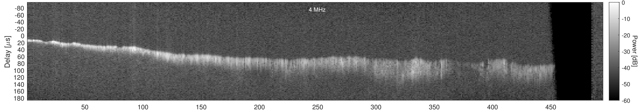
Orbit 5486, Window, Channel 2, Chapman
