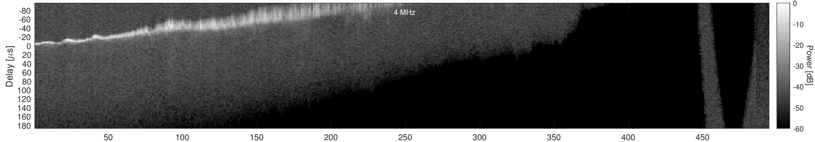
Orbit 5486, Window, Channel 2, Optimized
