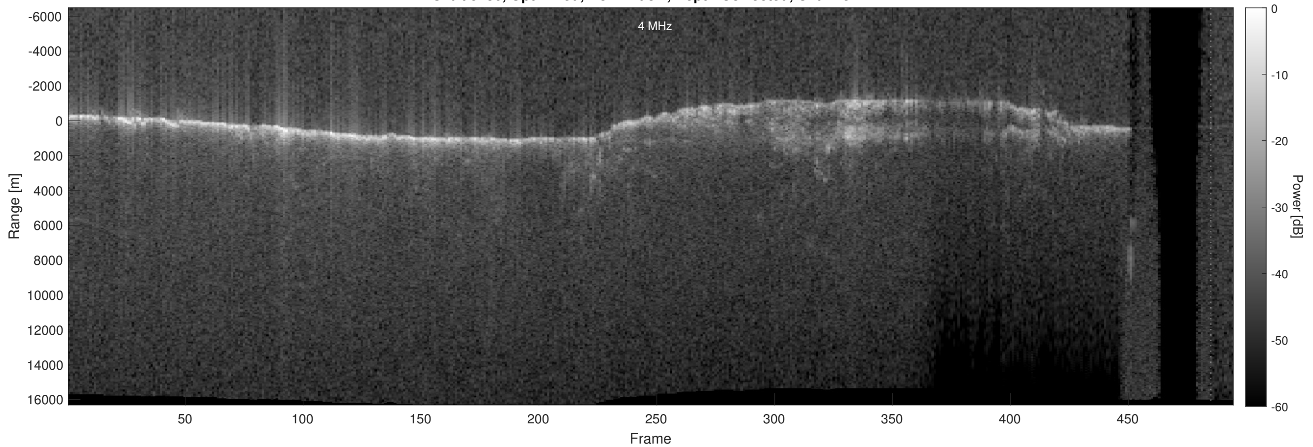
Orbit 5486, Optimized, No Window, Depth-Corrected, Channel 2
