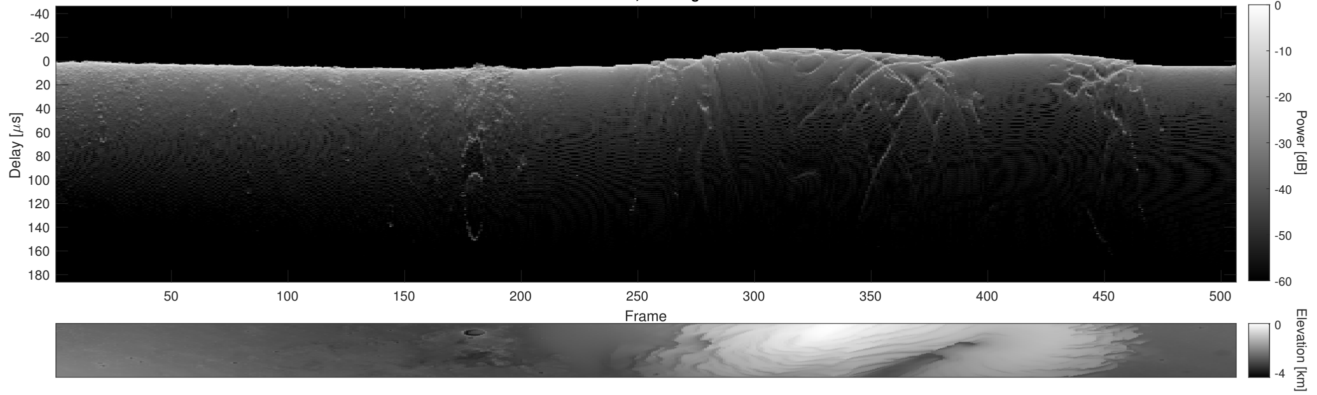
Orbit 5490, Cluttergram
