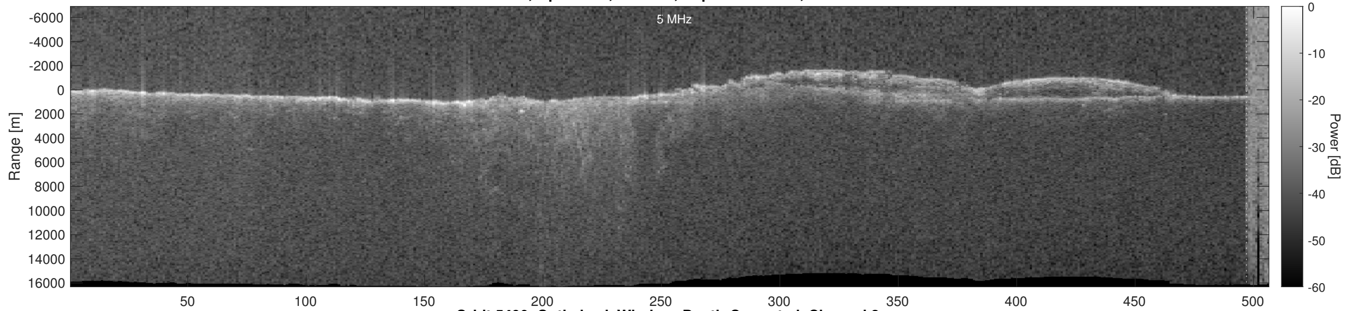
Orbit 5490, Optimized, Window, Depth-Corrected, Channel 2
