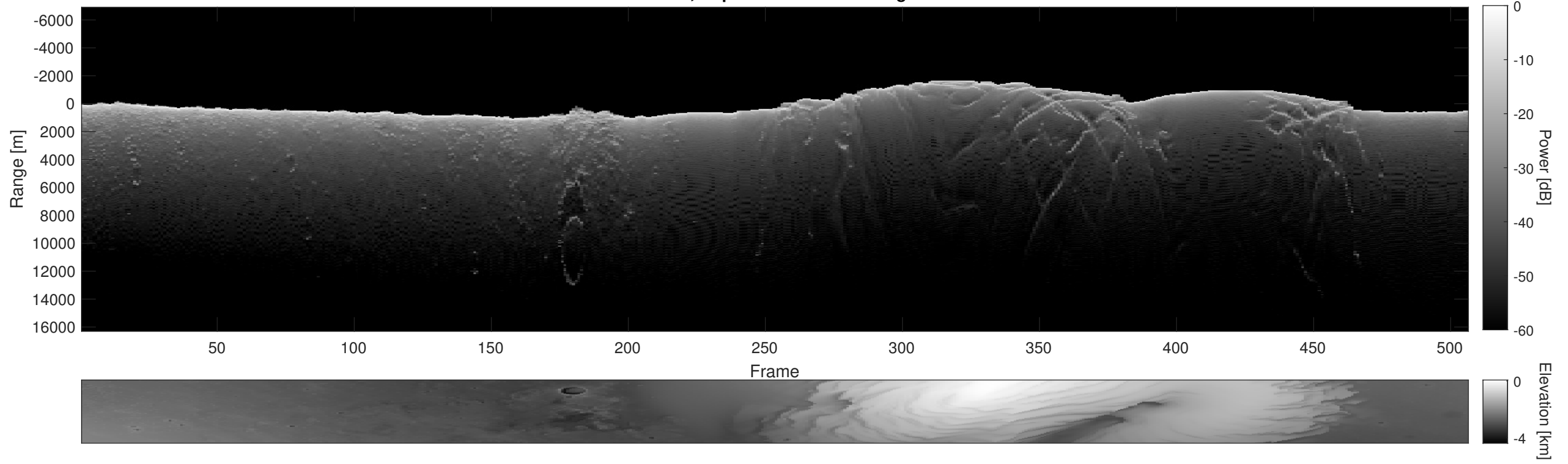
Orbit 5490, Depth-Corrected Cluttergram
