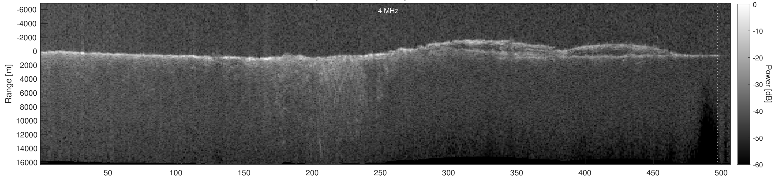
Orbit 5490, Depth-Corrected Cluttergram
