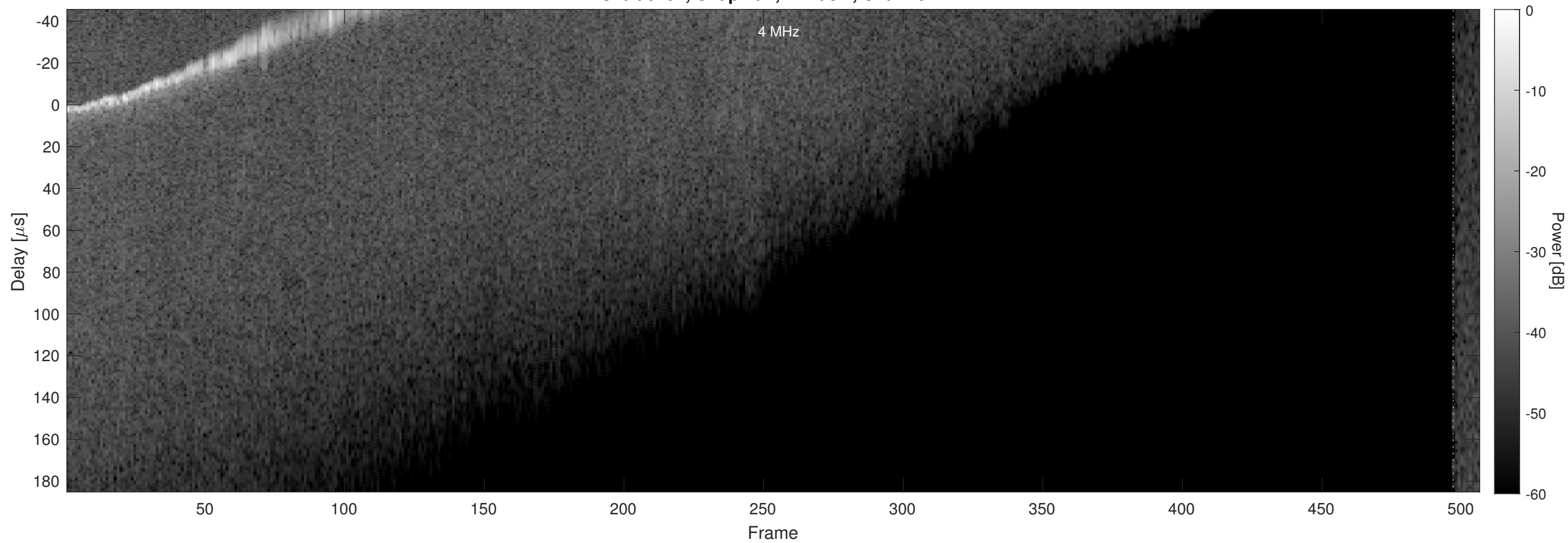
Orbit 5491, Chapman, Window, Channel 2
