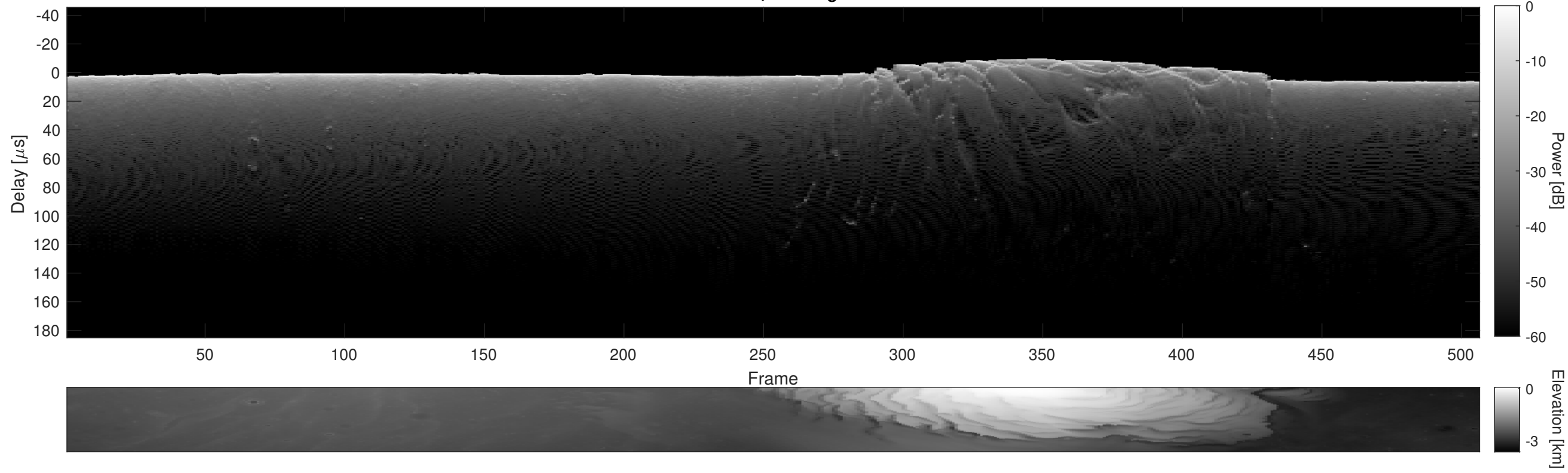
Orbit 5491, Cluttergram
