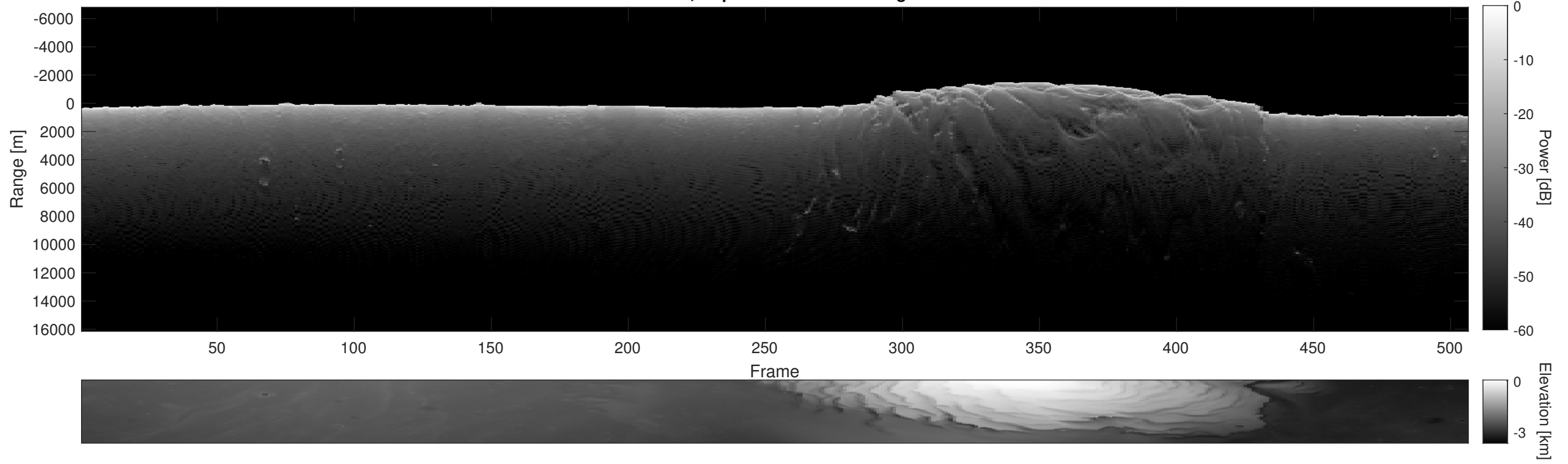
Orbit 5491, Depth-Corrected Cluttergram
