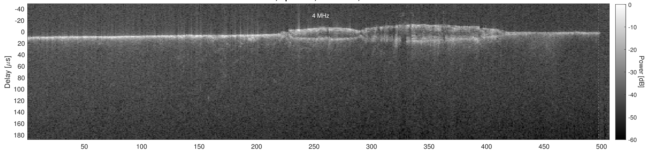
Orbit 5496, Cluttergram
