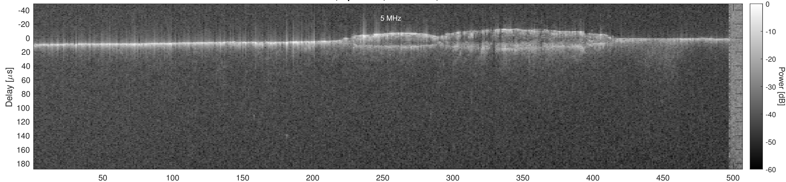
Orbit 5496, Optimized, No Window, Channel 2
