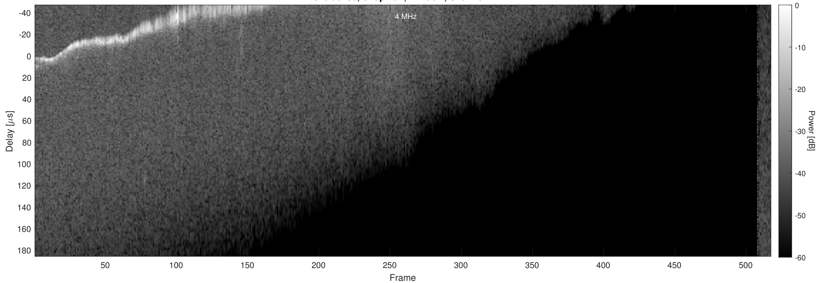
Orbit 5498, Chapman, Window, Channel 2
