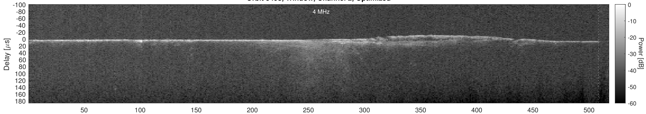
Orbit 5498, Cluttergram
