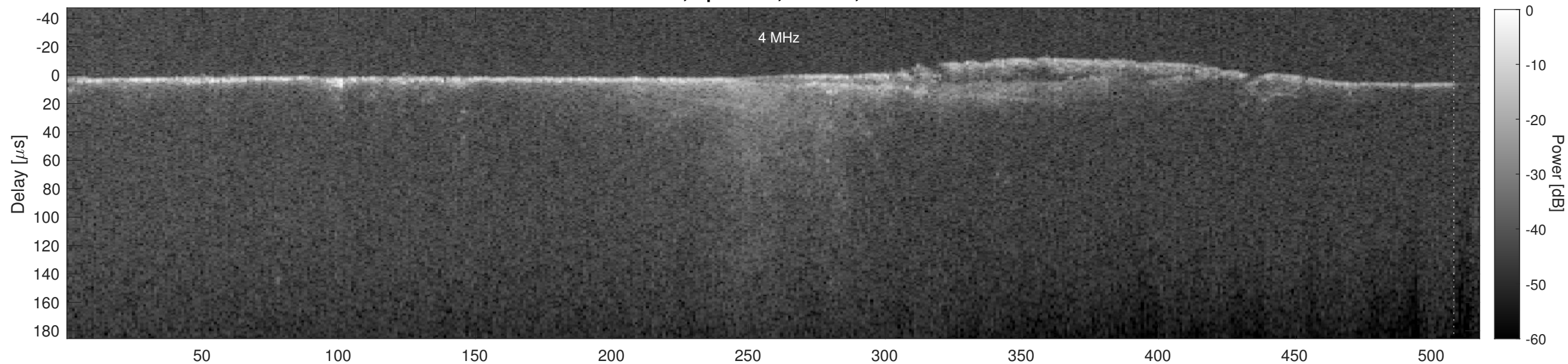
Orbit 5498, Cluttergram
