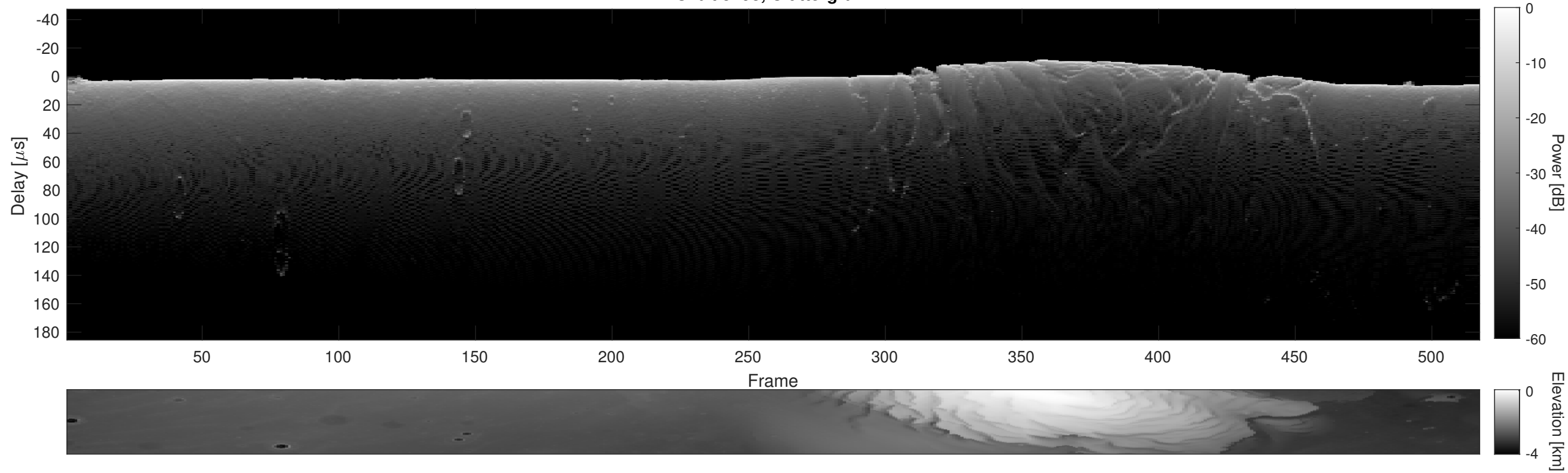
Orbit 5498, Cluttergram
