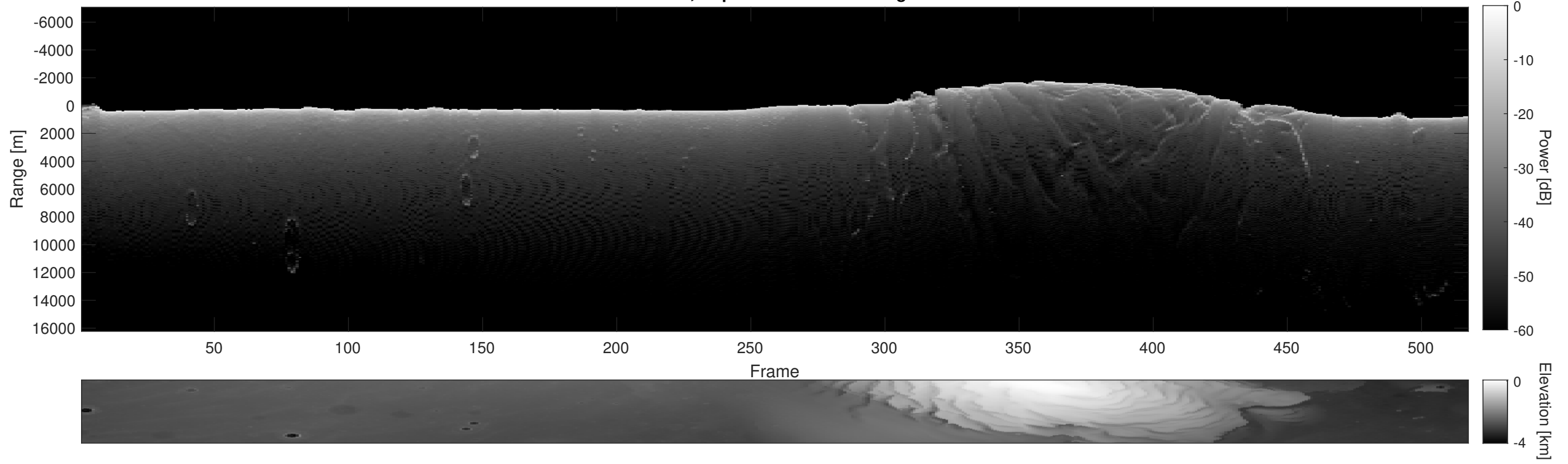
Orbit 5498, Depth-Corrected Cluttergram
