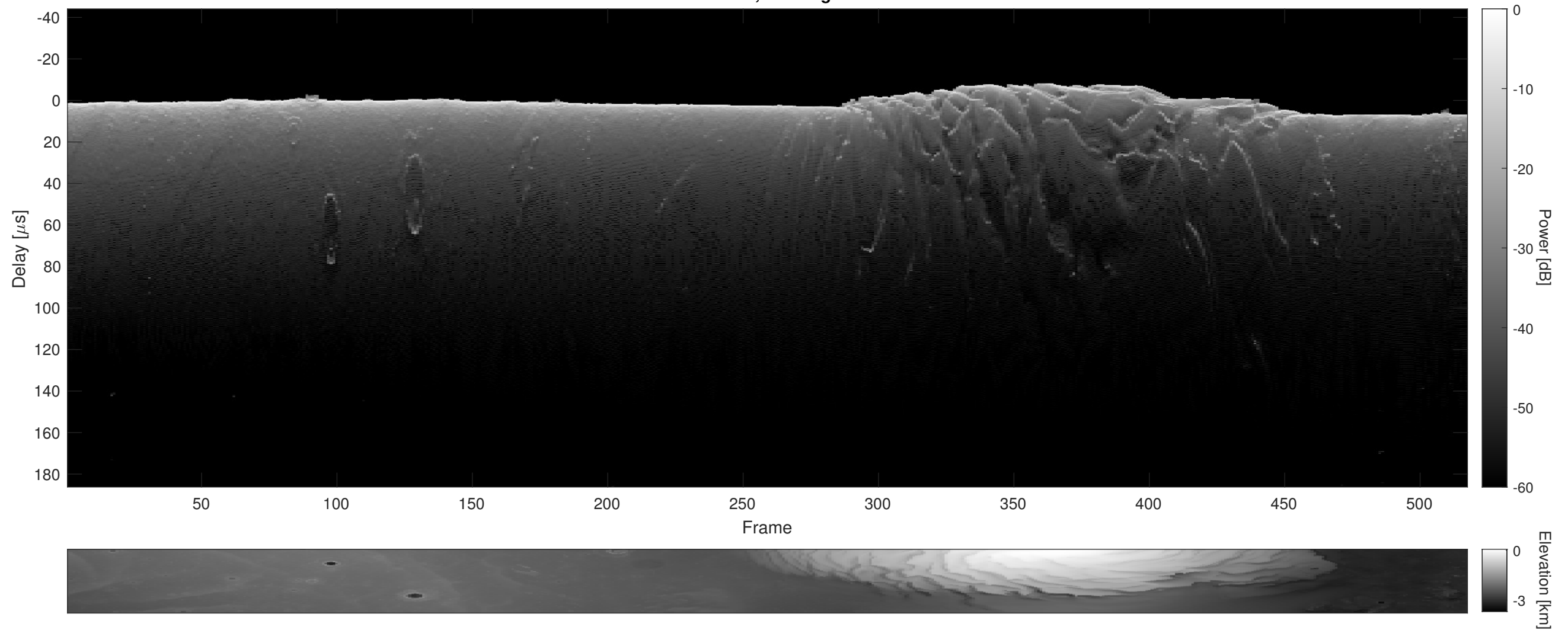
Orbit 5502, Cluttergram
