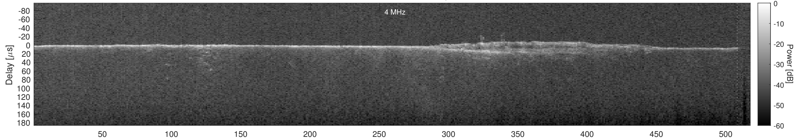
Orbit 5502, Cluttergram
