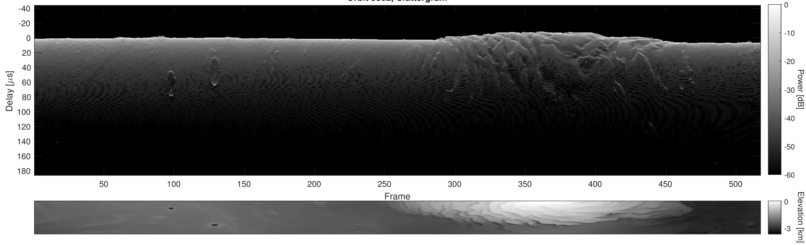
Orbit 5502, Cluttergram
