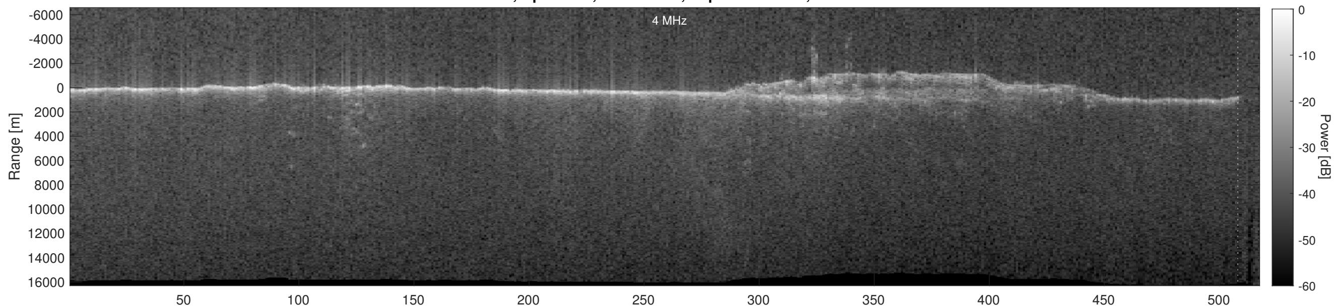
Orbit 5502, Depth-Corrected Cluttergram
