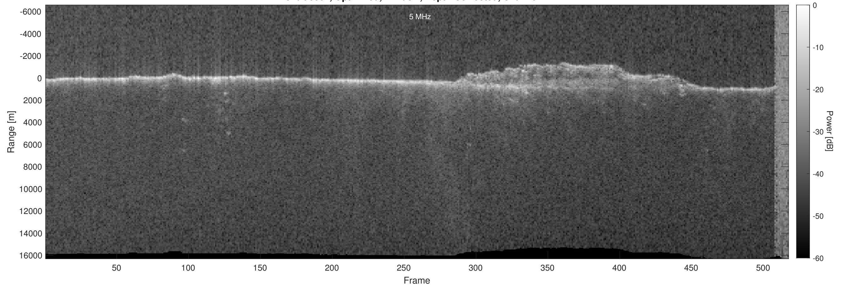
Orbit 5502, Optimized, Window, Depth-Corrected, Channel 2
