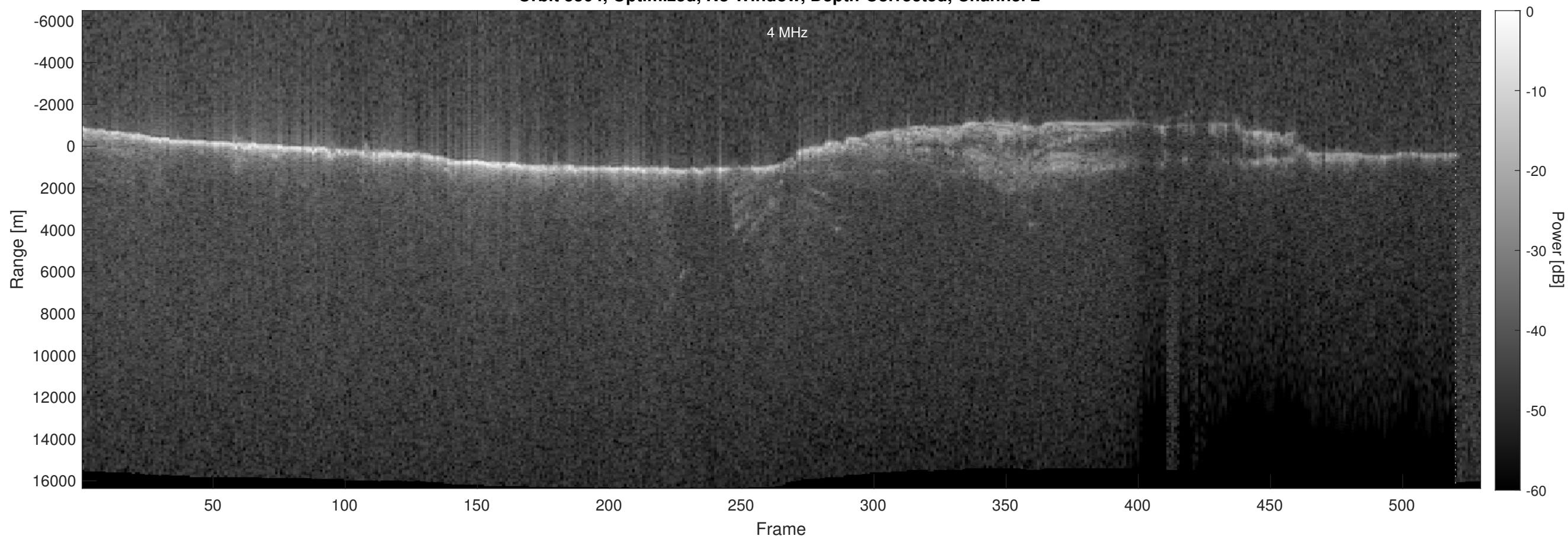
Orbit 5504, Optimized, No Window, Depth-Corrected, Channel 2
