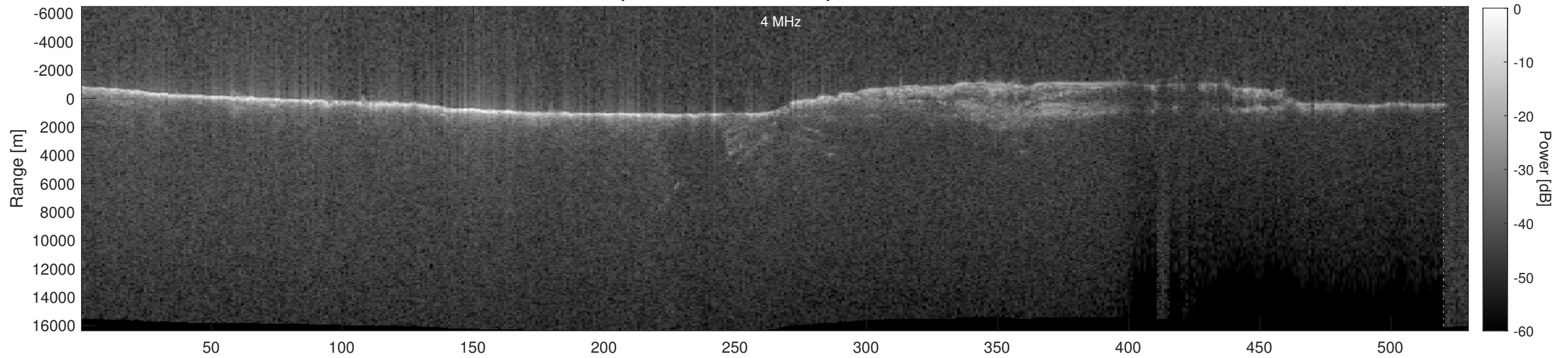
Orbit 5504, Depth-Corrected Cluttergram
