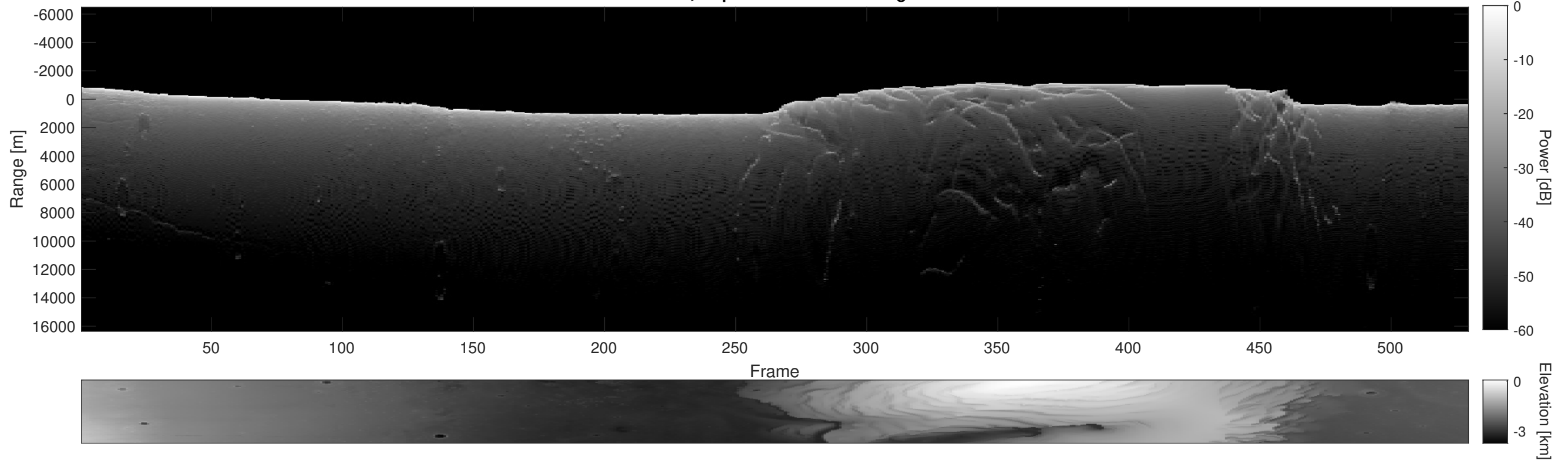
Orbit 5504, Depth-Corrected Cluttergram
