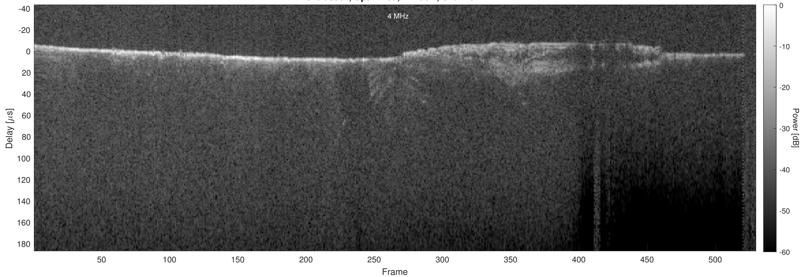
Orbit 5504, Optimized, Window, Channel 2
