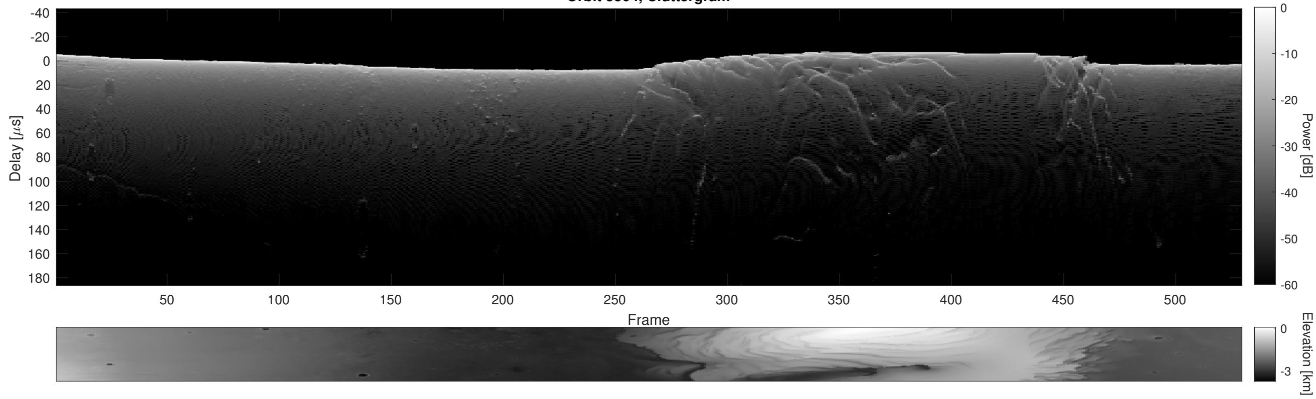
Orbit 5504, Cluttergram
