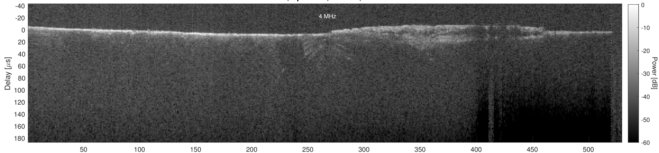
Orbit 5504, Cluttergram
