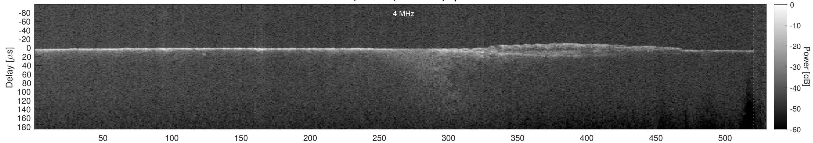
Orbit 5509, Cluttergram
