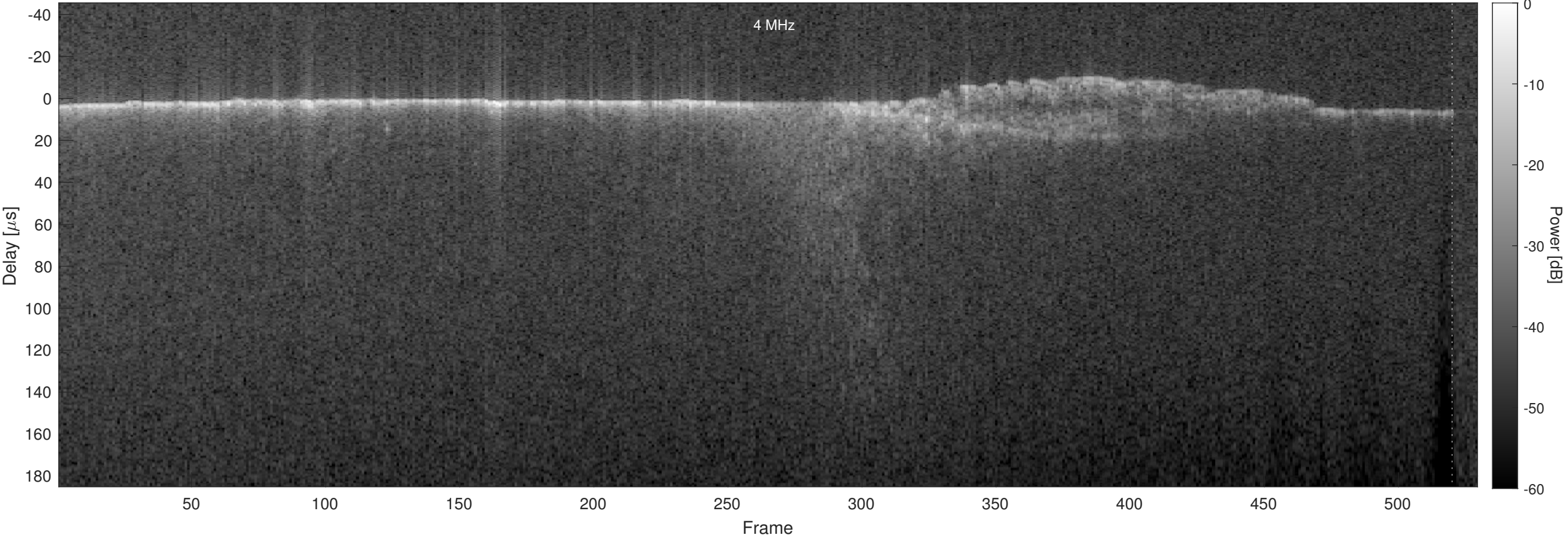
Orbit 5509, Optimized, No Window, Channel 2
