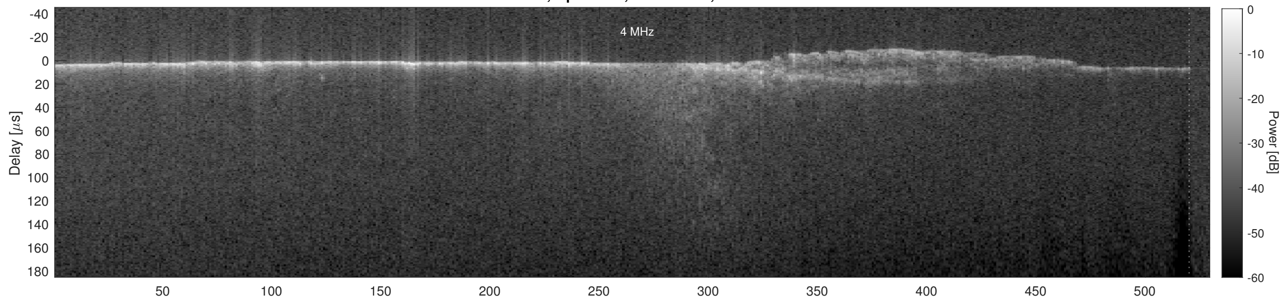
Orbit 5509, Cluttergram
