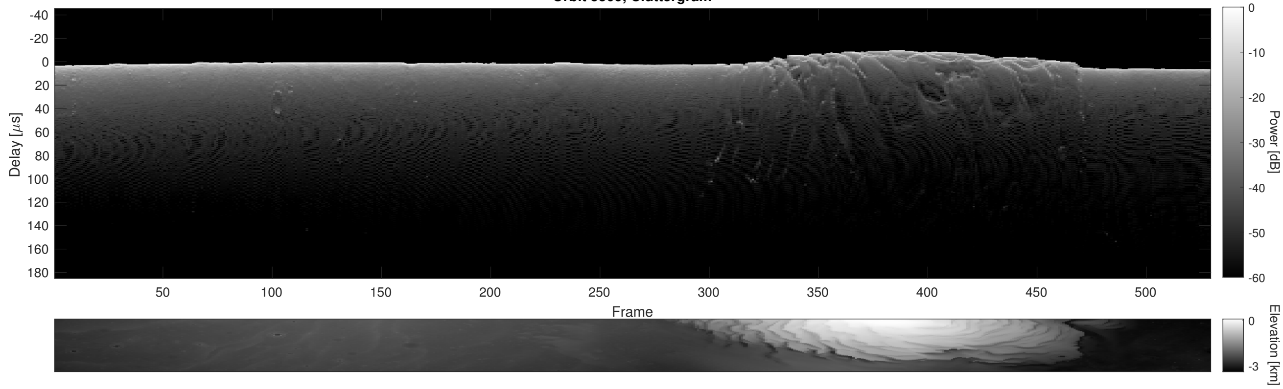
Orbit 5509, Cluttergram
