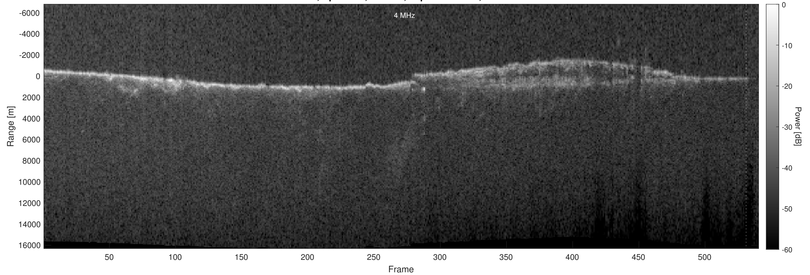
Orbit 5511, Optimized, Window, Depth-Corrected, Channel 2
