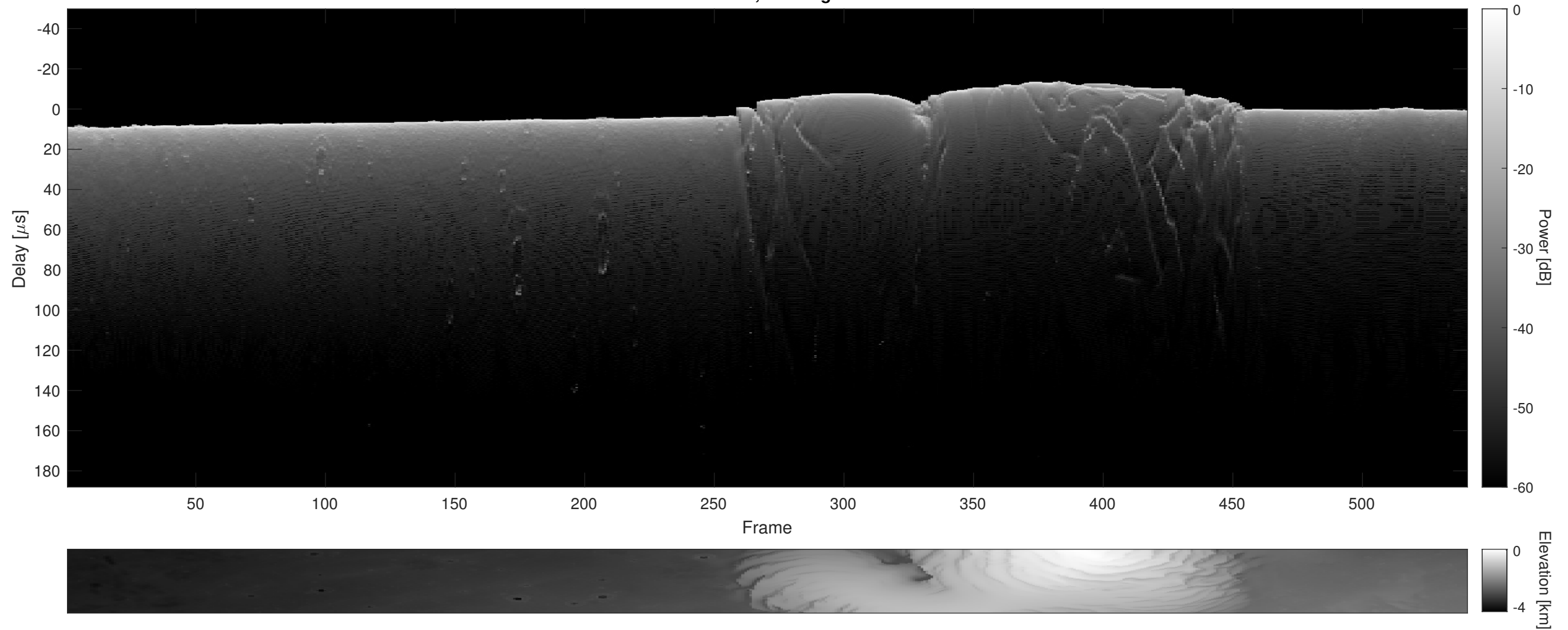
Orbit 5514, Cluttergram
