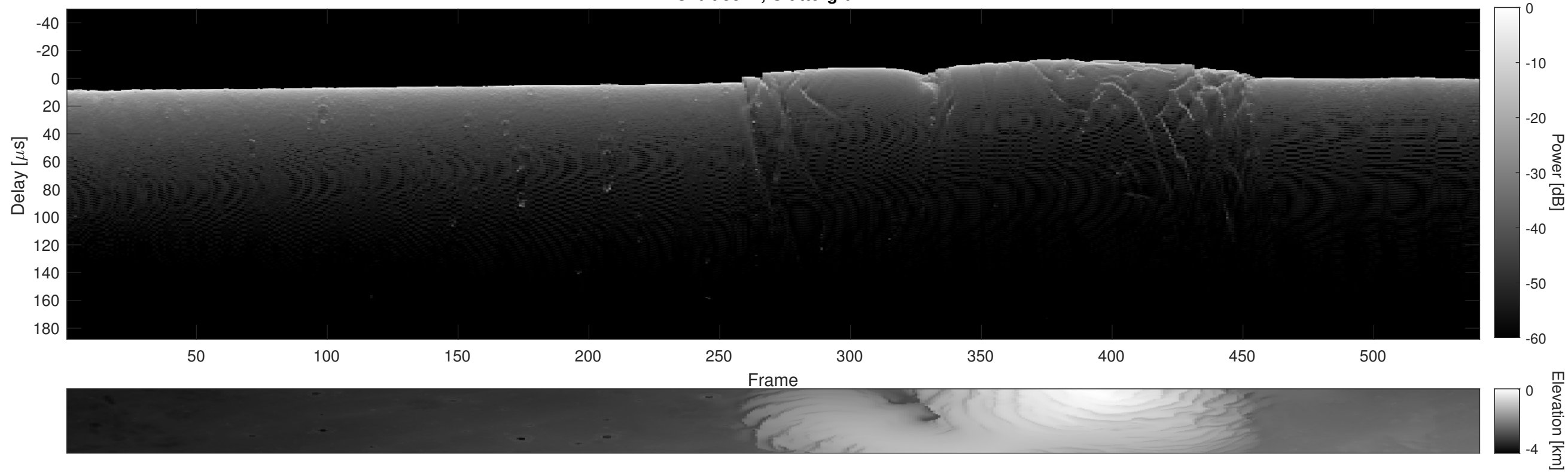
Orbit 5514, Cluttergram
