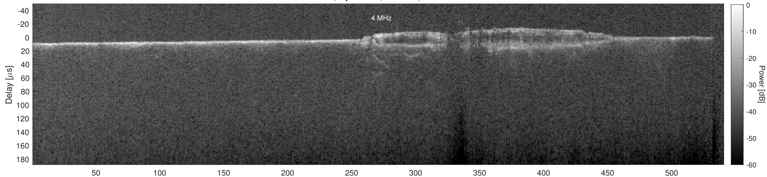
Orbit 5514, Cluttergram
