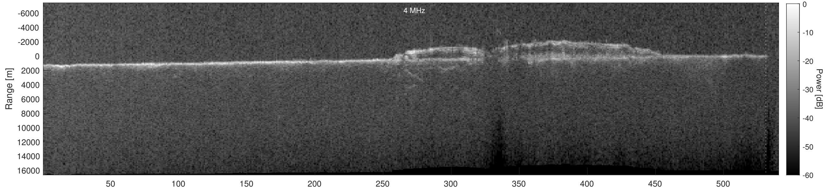
Orbit 5514, Depth-Corrected Cluttergram
