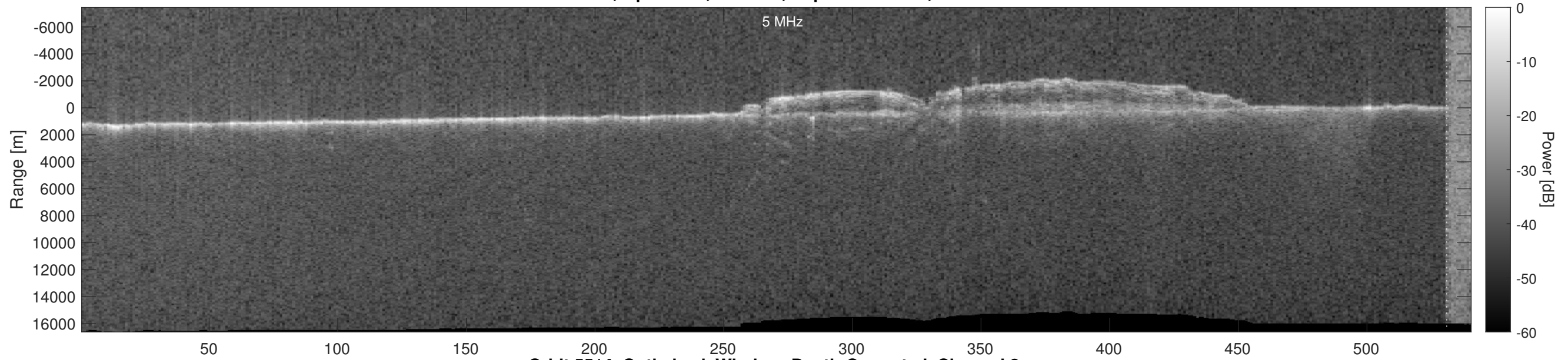
Orbit 5514, Optimized, Window, Depth-Corrected, Channel 2
