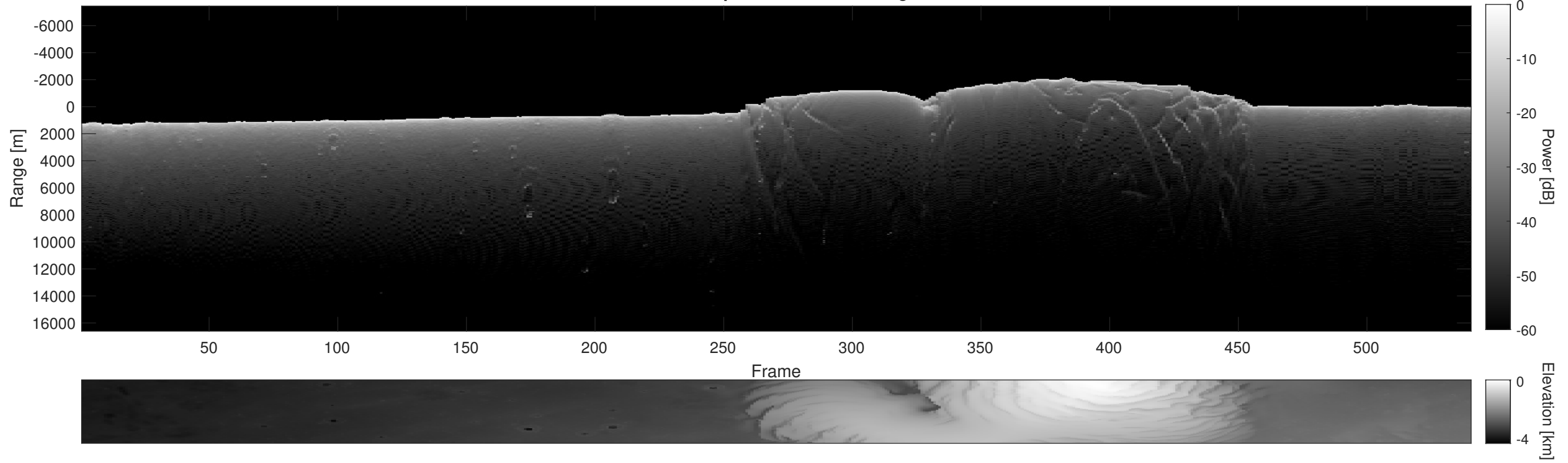
Orbit 5514, Depth-Corrected Cluttergram
