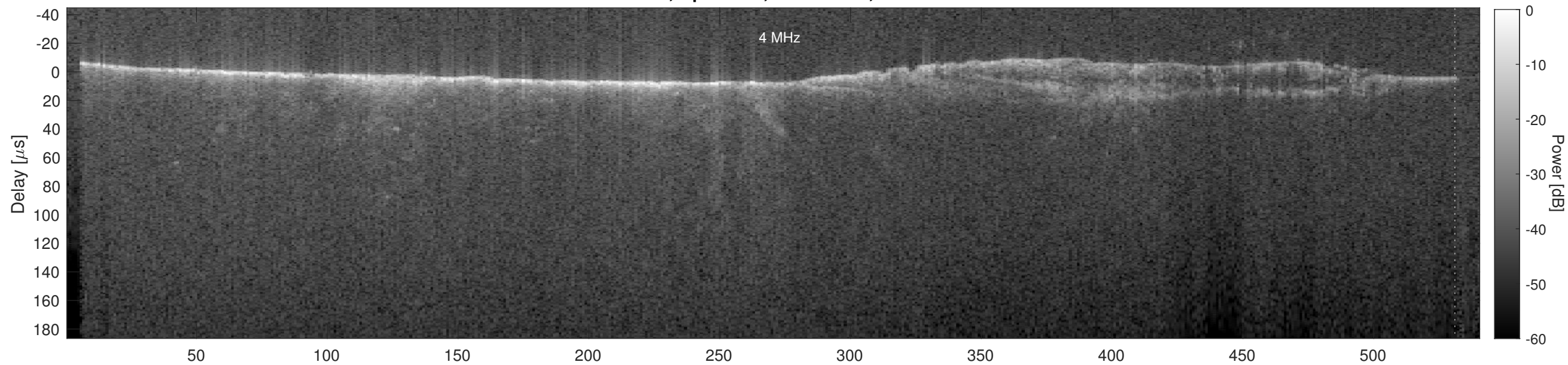
Orbit 5515, Cluttergram
