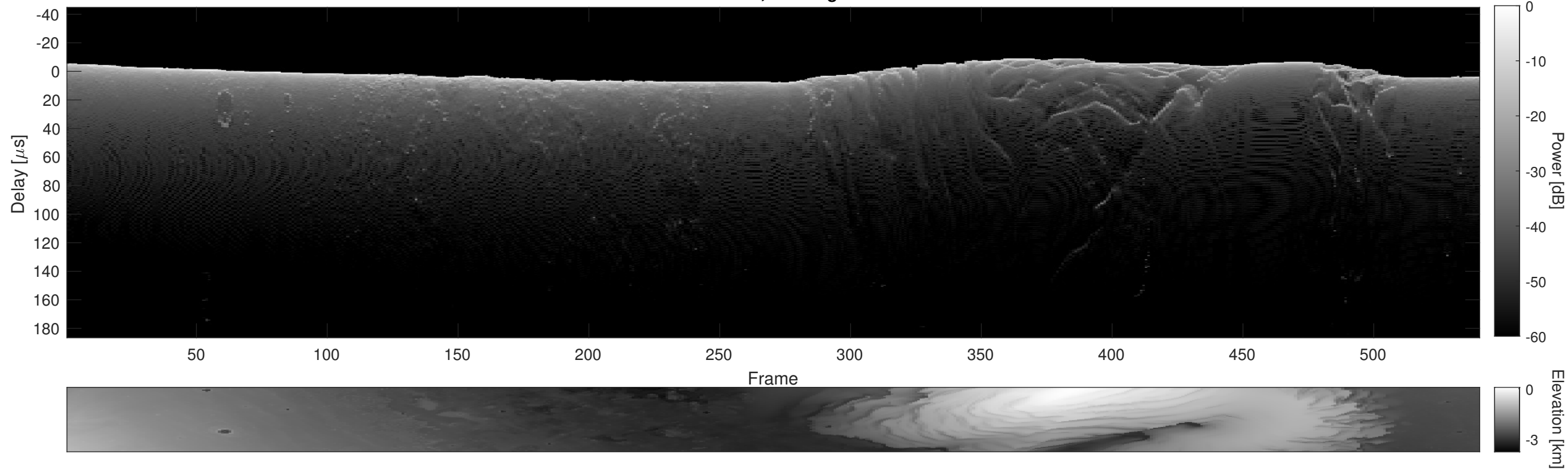
Orbit 5515, Cluttergram
