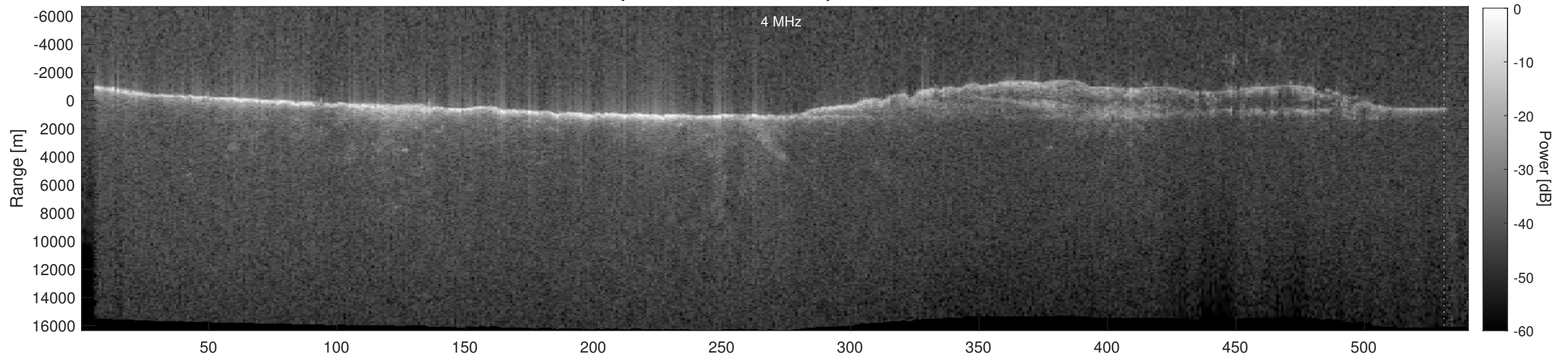
Orbit 5515, Depth-Corrected Cluttergram
