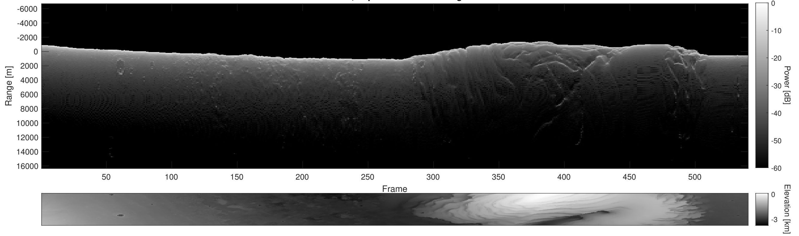
Orbit 5515, Depth-Corrected Cluttergram
